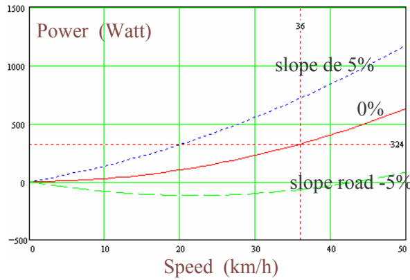
Figure 2: Motive power vs speed for different slopes ( M=100kg , f=0.25 N/km.h^{-1} )
